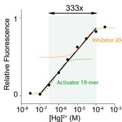
Figure 5. Extending the dynamic range of metal binding switches using a mixture of an allosteric activator and an allosteric inhibitor. While the switch in the presence of a single allosteric effector shows a limited dynamic range (only 8-fold in target concentration; see dashed curves), this same dynamic range is widened to almost 3 orders of magnitude in the presence of the activator/inhibitor mixture (solid line). Here the switch concentration was held at 10 nM, and the activator (21-base) and inhibitor (20-base) concentrations were held at 7 and 3 nM respectively (see SI for details).
